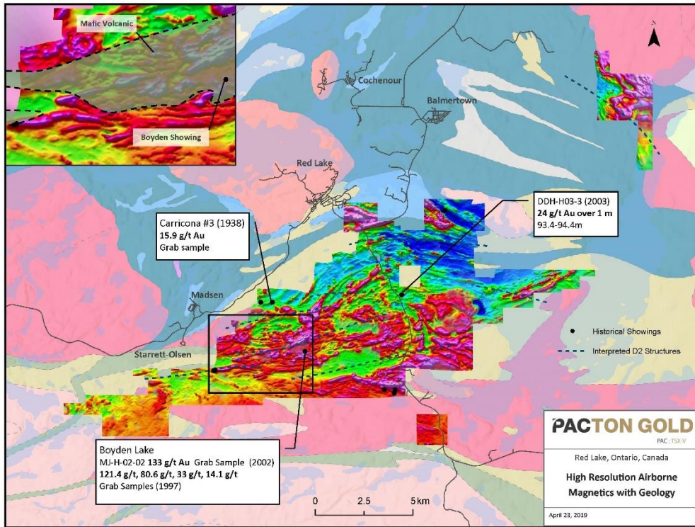
Figure 1. Pacton Gold’s Red Lake Property with New Magnetic Survey. Inset over western half of property with intensely folded basalt units cut by D2 structures.
