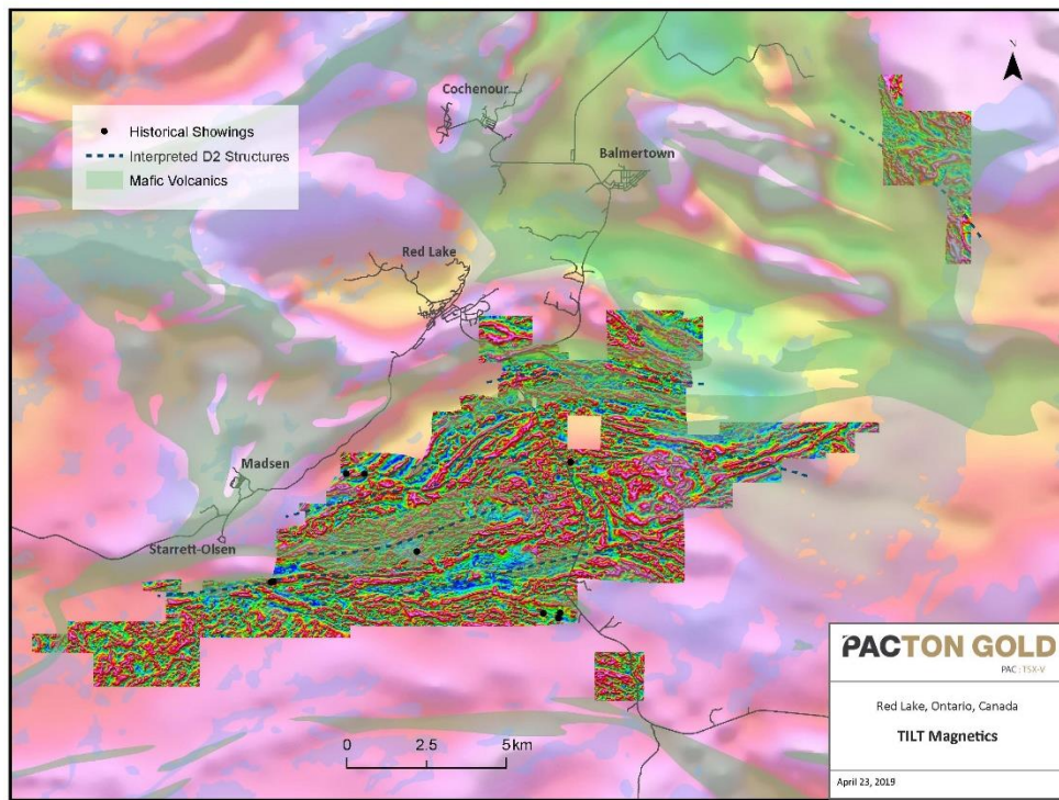
Figure 2. Pacton Gold’s Red Lake Property with New Magnetic Survey (Tilt variation) showing detailed structure.
